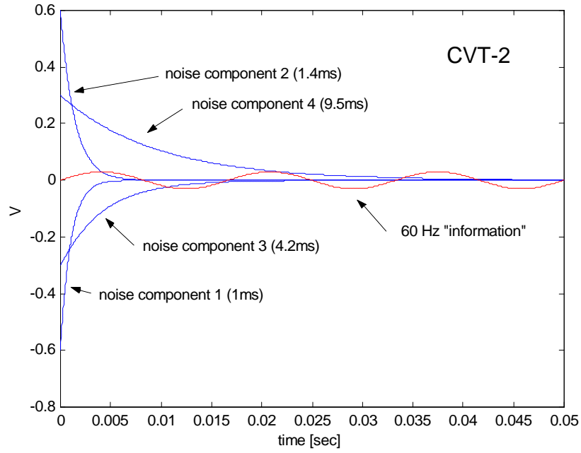
Figure 5. Comparison of the CVT noise with a low 60Hz signal for the extra high-C CVT.
