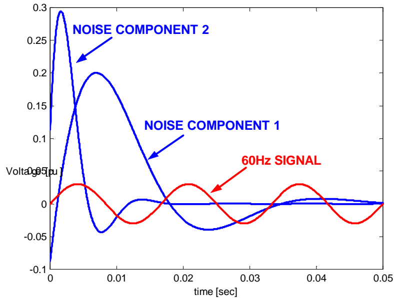
Figure 7. Illustration of the signal-to-noise ratio for the CVT transients (CVT-1 fault at zero crossing) and high SIRs (30).
