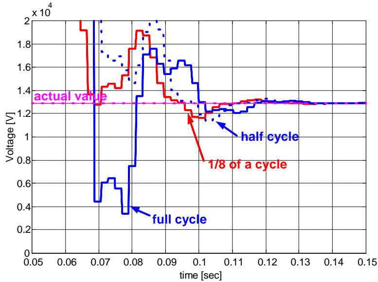
Figure 9. Voltage magnitude estimated using various window lengths for a fault at the reach point with the SIR of 30 and CVT-1 as a voltage source (90 deg inception angle, fault at 50 msec).
