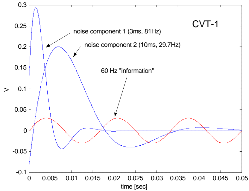
Figure 6. Comparison of the CVT noise with a low 60Hz signal for the high-C CVT.
