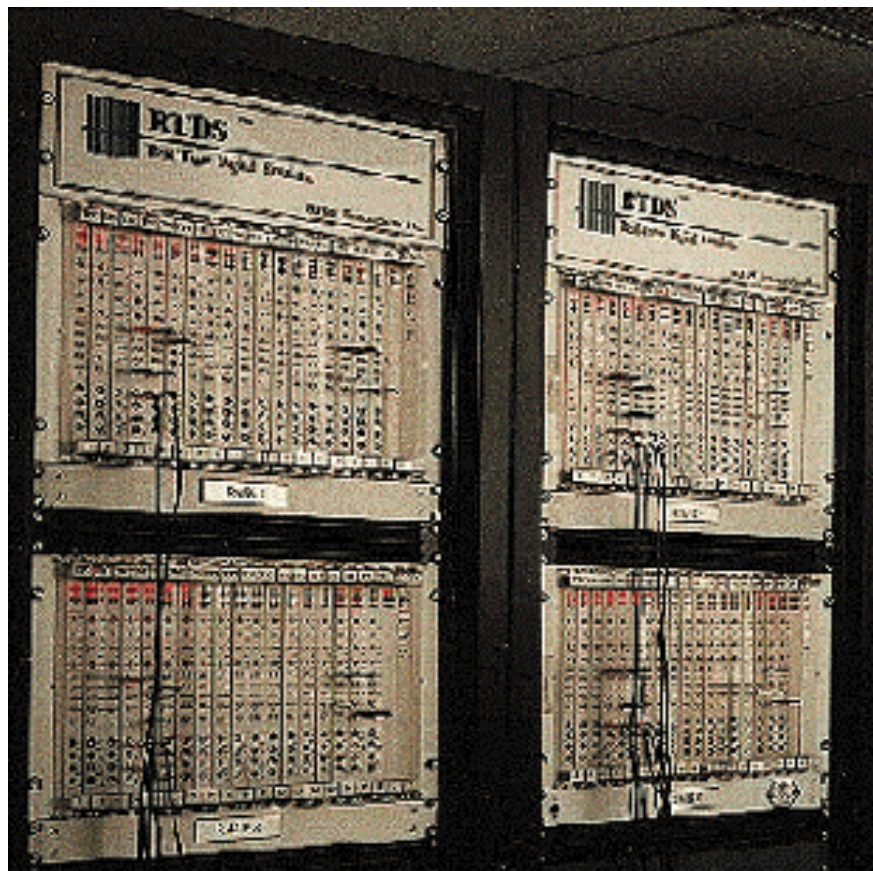
Figure 17. RTDS hardware used in testing.
