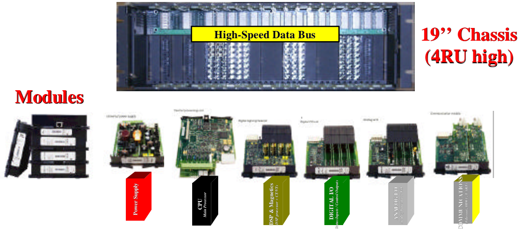
Figure 16. Actual relay architecture.
