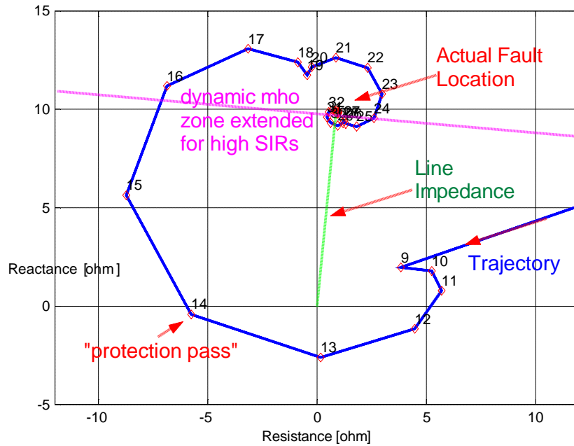
Figure 10. Impedance locus may "fly" below the line impedance vector (CVT-1, SIR=30, 90 deg fault inception angle, the numbers mark protection passes being 2msec apart).
