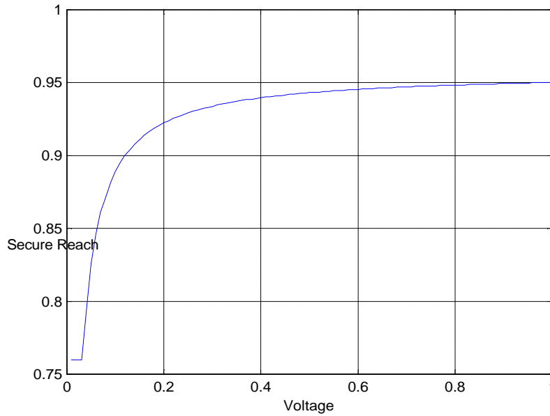
Figure 14. Inner zone 1 reach as a function of the voltage magnitude.
