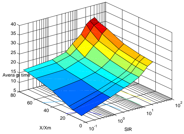
Figure 18. Average operating times of the new algorithm (MATLAB).
