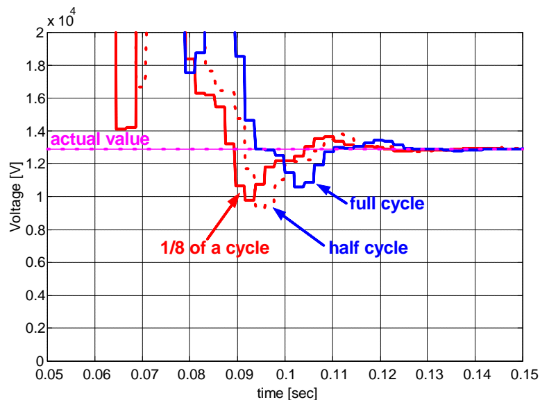
Figure 8. Voltage magnitude estimated using various window lengths for a fault at the reach point with the SIR of 30 and CVT-1 as a voltage source (0 deg inception angle, fault at 54 msec).
