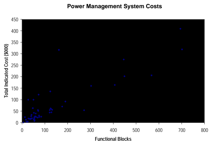
Range of Total Installed Cost Fig. 4
