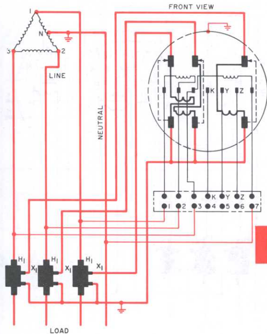
Type V-66-S, 240-volt, Class 10 or 20 or EV-6-S Class 20 meter with CT's. Bottom-connected 13-jaw socket with circuit-closing devices
