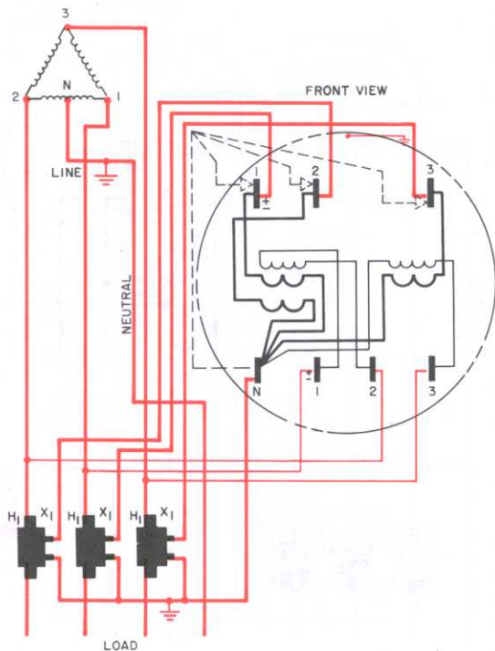
Type V-66-S, 240- or 480-volt, Class 10 or 20 or EV-6-S Class 20 meter with CT's; 7-jaw socket with circuit-closing devices
