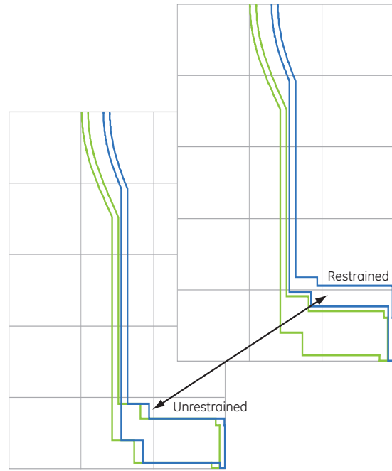
Advanced ZSI allows Instantaneous ZSI to withstand ratings 100kA of selectivity & 3 cycle clearing, simultaneously
