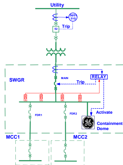
Figure 5 - Architecture
