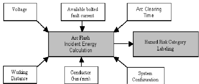
Figure 1 – Incident Energy Calculation
